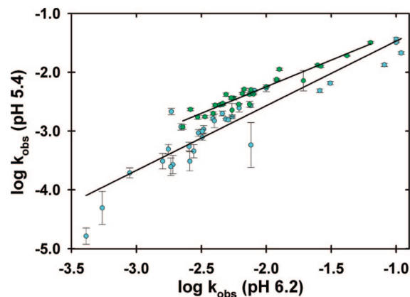
Figure 2. The I29A/I37H variant exchanges according to the EX2 mechanism. Linear regression yields slopes and R^2 values of 0.91 \pm 0.5 and 0.92 in dilute solution (green) and 1.10 \pm 0.08 and 0.86 in 300 g/L PVP40 (cyan), respectively. The error bars represent the standard errors for the averages from three trials collected at pH 5.4.
