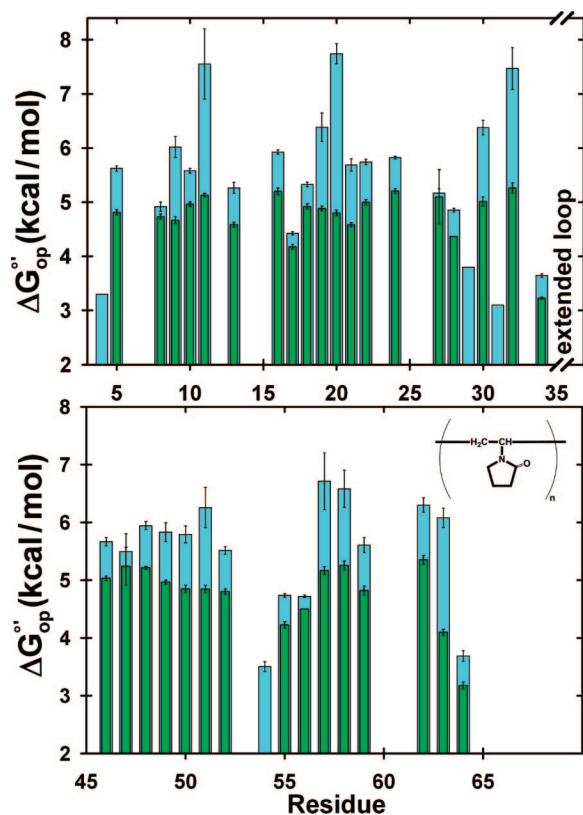
Figure 4. Macromolecular crowding with PVP40 stabilizes the I29A/I37H variant of CI2 relative to dilute solution. Values of \Delta G_{\text{op}}^{\text{o}} in 300 g/L PVP40 (cyan) and dilute solution (green) are plotted versus residue number. The height of each bar represents the average from three trials. The error bars represent the standard deviation. Conditions: 700–800 \mu\text{M} variant protein, 50 mM acetate buffer in \text{D}_2\text{O} , pH 5.4. The inset shows the backbone structure of PVP.
