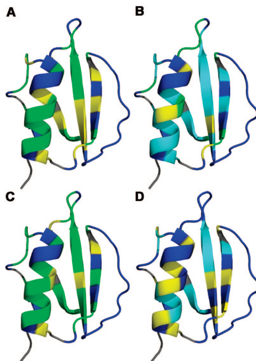
Figure 5. Ribbon structure of wild-type CI2 (PDB, 2CI2) colored by \Delta G_{\text{op}}^{\text{o}} for the I29A/I37H variant in (A) dilute solution, (B) 300 g/L PVP40, and (C) 100 g/L NEP [blue: \Delta G_{\text{op}}^{\text{o}} < 3.0 \text{ kcal/mol} ; green: < 3.0 \text{ kcal/mol} \Delta G_{\text{op}}^{\text{o}} < 5.0 \text{ kcal/mol} ; yellow: 5.0 \text{ kcal/mol} < \Delta G_{\text{op}}^{\text{o}} < 5.5 \text{ kcal/mol} ; cyan: 5.5 \text{ kcal/mol} < \Delta G_{\text{op}}^{\text{o}} < 8.0 \text{ kcal/mol} ]. (D) \Delta G_{\text{op}}^{\text{o}} was measured in 0, 50, 100, and 300 g/L PVP40, and \delta\Delta G_{\text{op}}^{\text{o}}/\delta[\text{PVP40}] values were superimposed onto the structure [blue: \delta\Delta G_{\text{op}}^{\text{o}}/\delta[\text{PVP40}] = 0 ; yellow: 0 < \delta\Delta G_{\text{op}}^{\text{o}}/\delta[\text{PVP40}] < 2.5 \times 10^{-3} \text{ (kcal/mol)/M} ; cyan: 2.5 \times 10^{-3} \text{ (kcal/mol)/M} < \delta\Delta G_{\text{op}}^{\text{o}}/\delta[\text{PVP40}] < 1.0 \times 10^{-2} \text{ (kcal/mol)/M} ]. Residues for which there are no data are colored gray.
